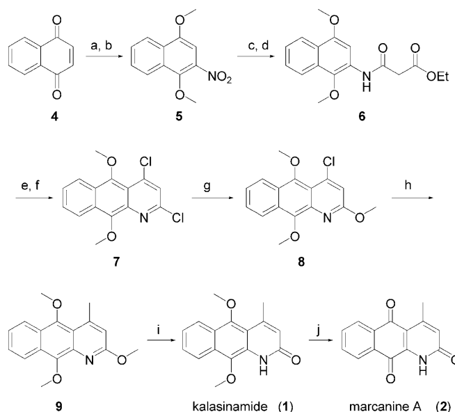
Scheme 2. Reagents and conditions: a) Pd/C, H 2 , THF; Me 2 SO 4 , reflux; b) HNO 3 , DCM; c) Ni, H 2 , 75% over three steps; d) malonic acid diethyl ester, 140°C, 3 h, 85%; e) 5% NaOH, 60°C, 3 h, 93%; f) POCl 3 , reflux, 2 h, 85%; g) MeONa, MeOH, RT, 3 d, 98%; h) MeMgCl, THF, MnCl 2 , 0°C, 2 h, 80%; i) TMSCl, NaI, MeCN, RT, 4 h, 95%; j) CAN, MeCN/H 2 O, RT, 4 h, 71%. DCM = dichloromethane, CAN = ceric ammonium nitrate.
