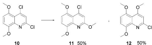
Scheme 3. Reagents and conditions: MeONa, MeOH, RT, 3 d.
