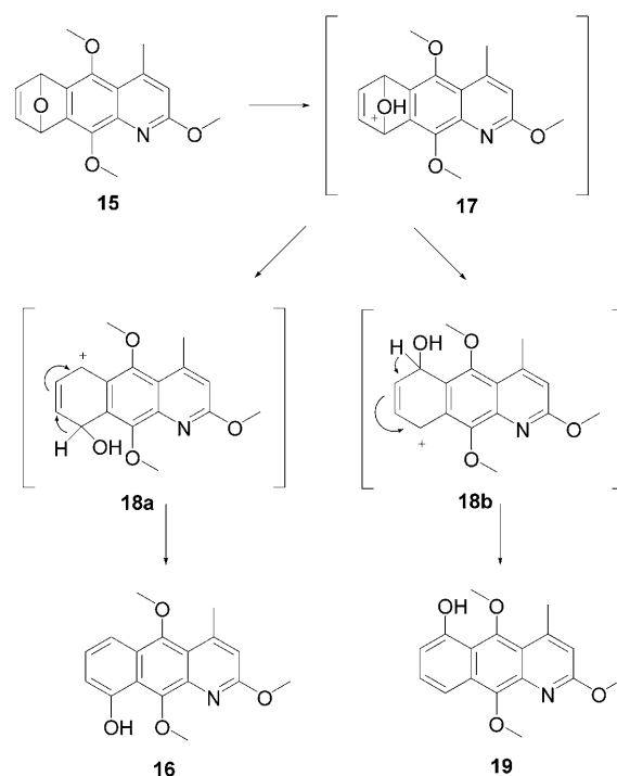
Scheme 6. Possible transition states and products of the acid-catalyzed ring opening of 15 .
