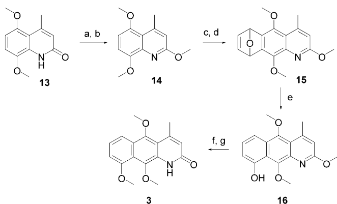
Scheme 5. Reagents and conditions: a) POCl 3 , reflux, 3 h; b) MeOK, MeOH, reflux, 5 h, 89 % over 2 steps; c) NBS, DCM, RT 2 h, 90%; d) LDA, THF, furan, −78 °C, 3 h, quant.; e) p -toluenesulfonic acid, THF, reflux, 20 h, 56%; f) MeI, NaH, DMF/THF, 96%; g) TMSCl, NaI, MeCN, RT 4 h, 85 %. NBS = N -bromosuccinimide, LDA = lithium diisopropylamide.
