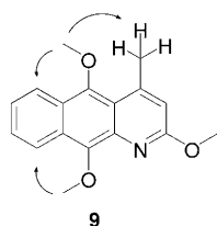
Scheme 4. NOE interactions observed for intermediate 9 .
