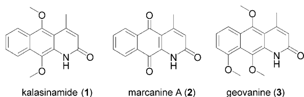
Scheme 1. Structures of naturally occurring azaanthracenones.
