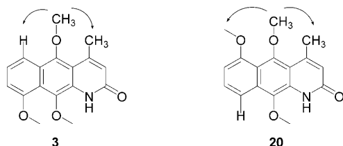
Scheme 7. Anticipated NOE interactions for isomers 3 and 20 .
